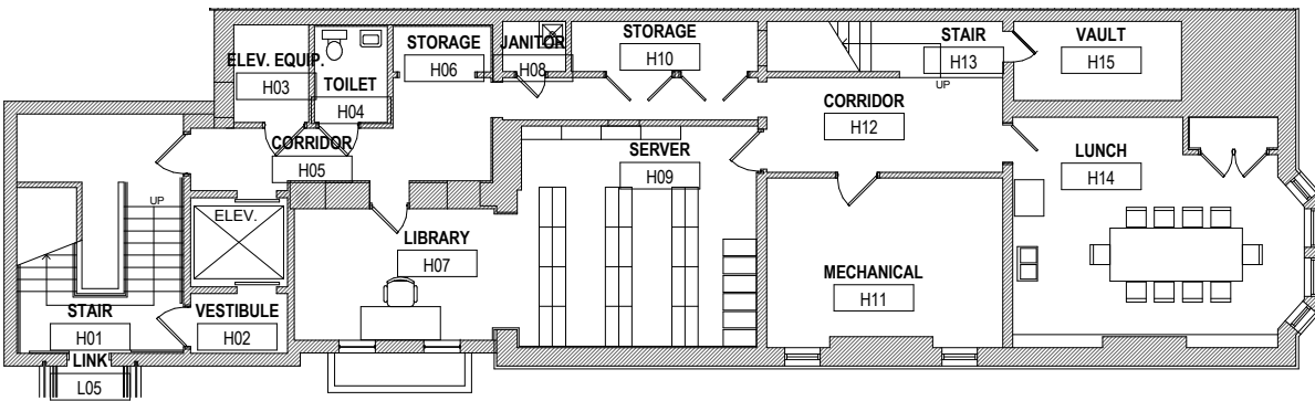
BASEMENT
