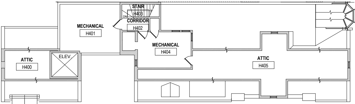
ATTIC LEVEL
