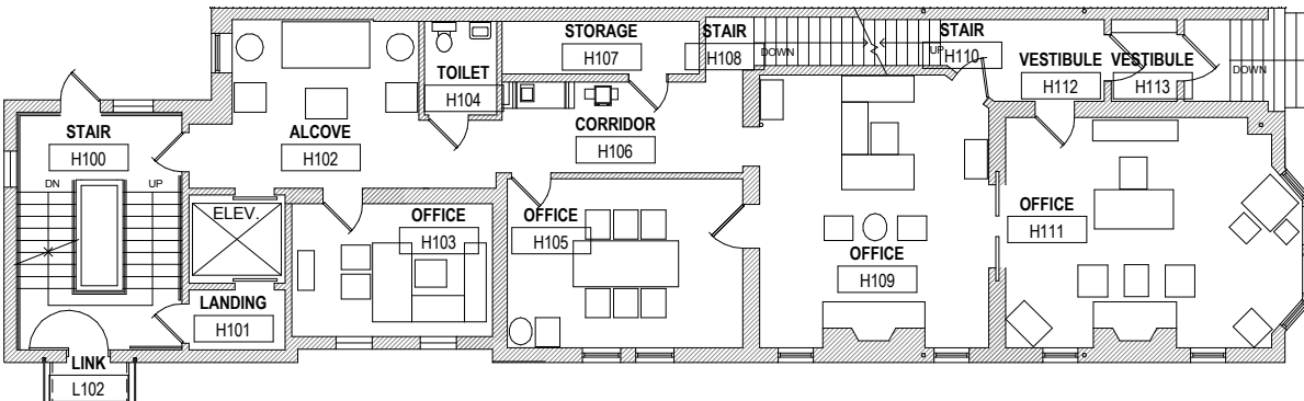
FIRST LEVEL
