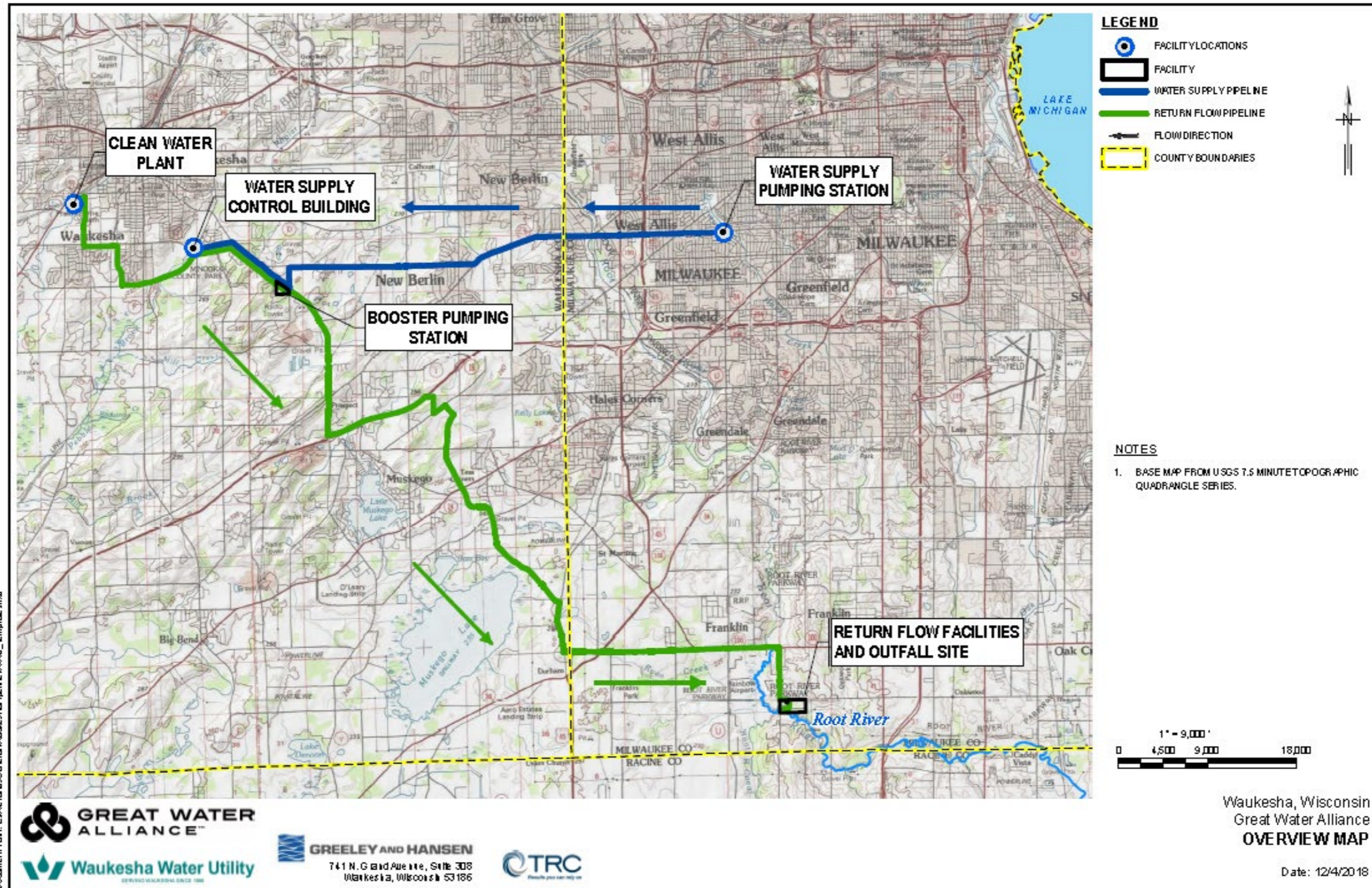
Figure 2-1 Program Schematic
